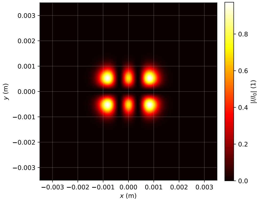
Intensity profile I(x, y, z = 0.637)/I_0 , P_{in}=0.5P_{cr} , artificial time
